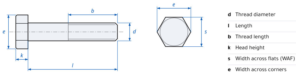
Hex Fit Bolt Long Thread DIN 609 - dimensions
