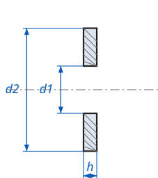
Sealing Ring Form A DIN 7603A - dimensions
