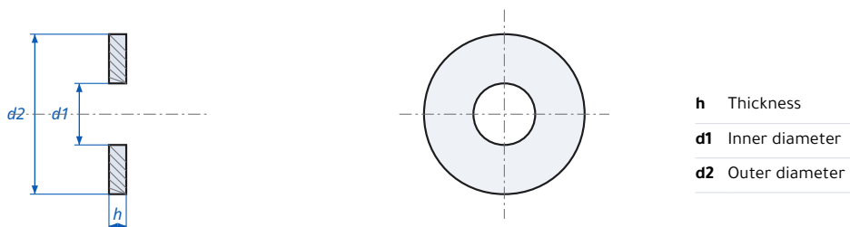
Flat Washer for Hex Bolts (Grade C) DIN 126 - dimensions
