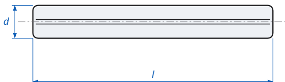
Slotted Spring Pin Light Duty DIN 7346 - dimensions
