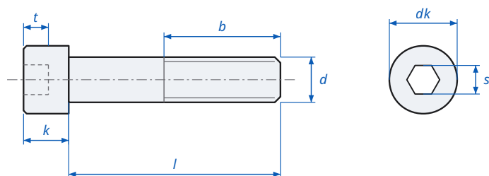
Hex Socket Head Cap Screw DIN 912 / ISO 4762 / ISO 12474 - dimensions
