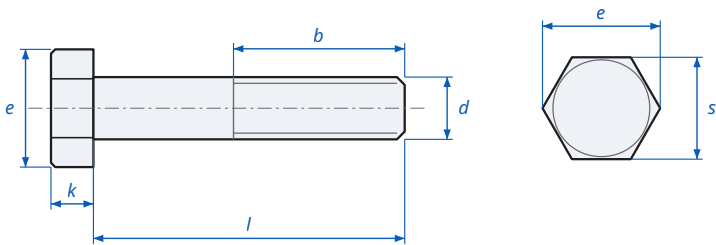
Hex Head Bolt Fine Thread DIN 960 / ISO 8765 - dimensions
