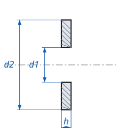
Flat Washer Small Series DIN 433 - dimensions
