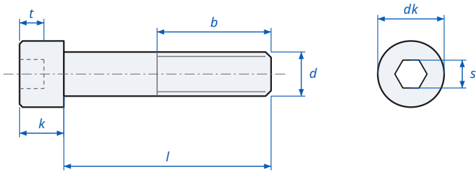
Socket Head Cap Screw ASME B18.3 - dimensions
