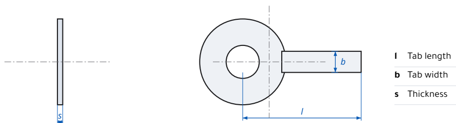
Tab Washer with Internal Tab DIN 462 - dimensions
