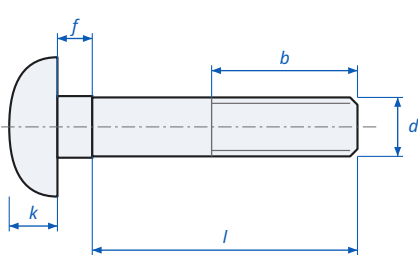
Mushroom Head Square Neck Bolt (Carriage Bolt) DIN 603 - dimensions
