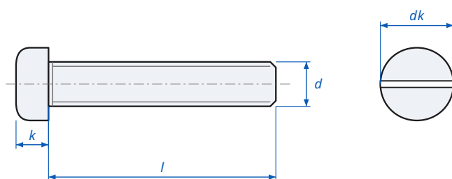
Slotted Pan Head Screw DIN 85 - dimensions
