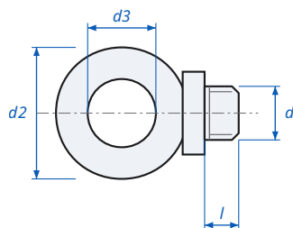
Lifting Eye Bolt DIN 580 - dimensions
