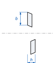
Spring Lock Washer Form B DIN 127B - dimensions
