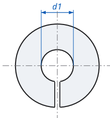
Spring Lock Washer Form B DIN 127B - dimensions
