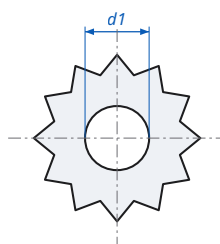
External Tooth Lock Washer DIN 6797A - dimensions
