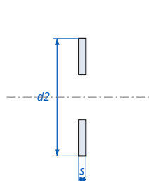
External Tooth Lock Washer DIN 6797A - dimensions
