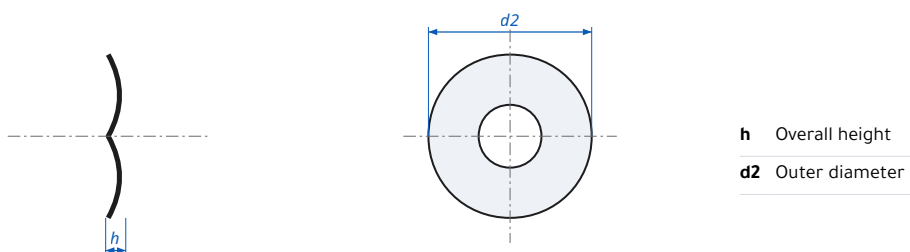
Wave Spring Washer DIN 137B - dimensions
