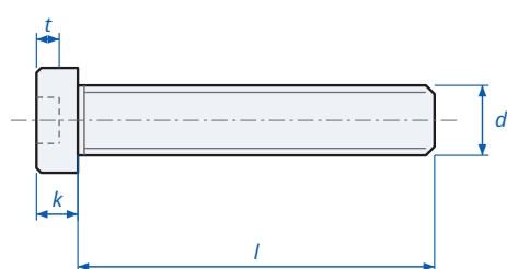
Low Head Socket Cap Screw (Holo-Krome) - dimensions
