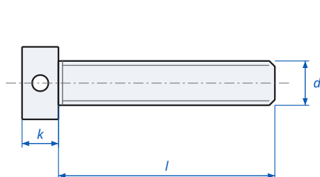
Slotted Capstan Screw DIN 404 - dimensions
