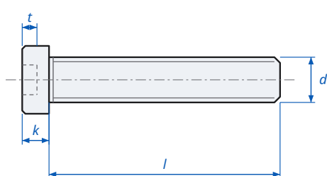
Low Head Socket Cap Screw DIN 7984 - dimensions
