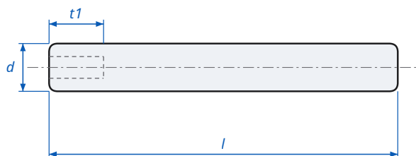
Parallel Pin with Internal Thread DIN 7979D - dimensions
