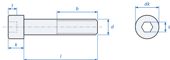
Hex Socket Head Cap Screw DIN 912 / ISO 4762 / ISO 12474 - dimensions
