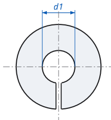
Spring Lock Washer Form B DIN 127B - dimensions
