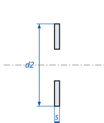
Countersunk Serrated Lock Washer DIN 6798V - dimensions
