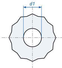
Countersunk Serrated Lock Washer DIN 6798V - dimensions
