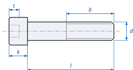
Hex Socket Head Cap Screw DIN 912 / ISO 4762 / ISO 12474 - dimensions
