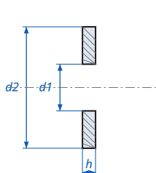
Washer for Steel Structures DIN 7989C - dimensions
