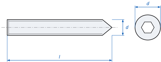
Socket Set Screw Cone Point ASME B18.3 - dimensions
