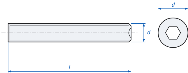
Socket Set Screw Cup Point ASTM F912 - dimensions
